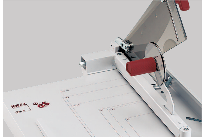
The automatic safety guard allows an unobstructed visual check of the entire cutting line and covers the blade in every position for safe cutting.
