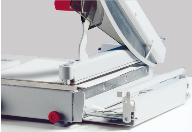
Exact gauges for precise cuts: The front gauge with integrated narrow strip cutting device is positioned via a calibrated rotary knob and can be locked in the preselected position.
