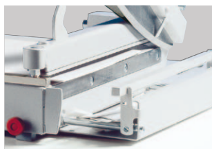
The front gauge with integrated narrow strip cutting device is positioned via a calibrated rotary knob.
