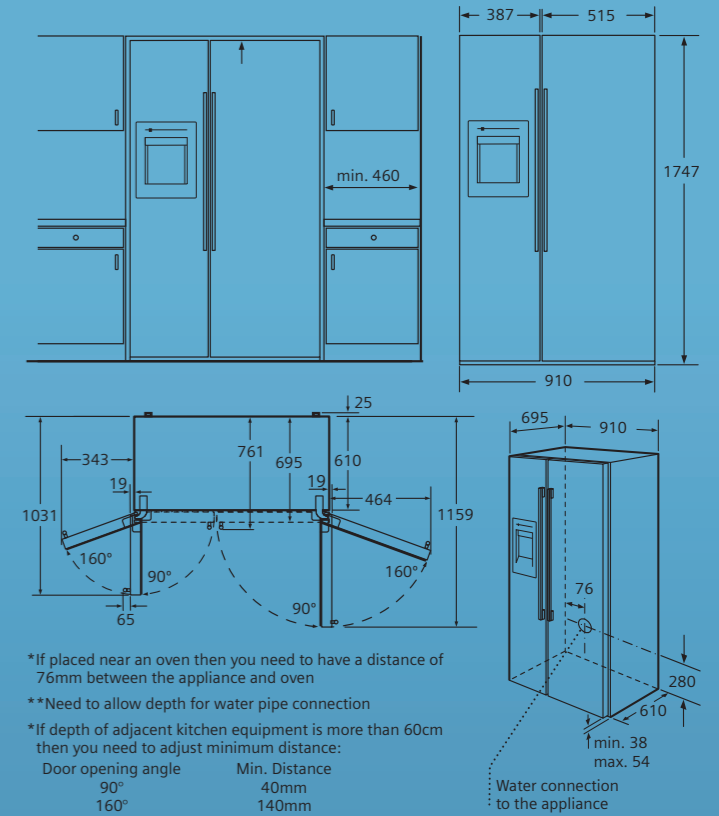
Measurements in mm
