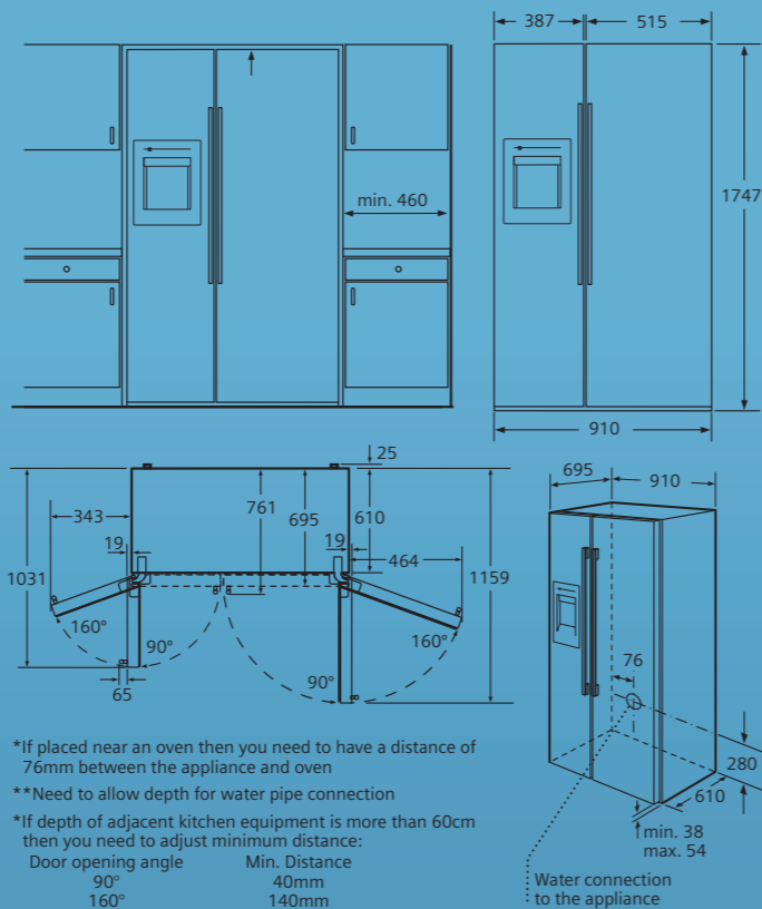
Measurements in mm
