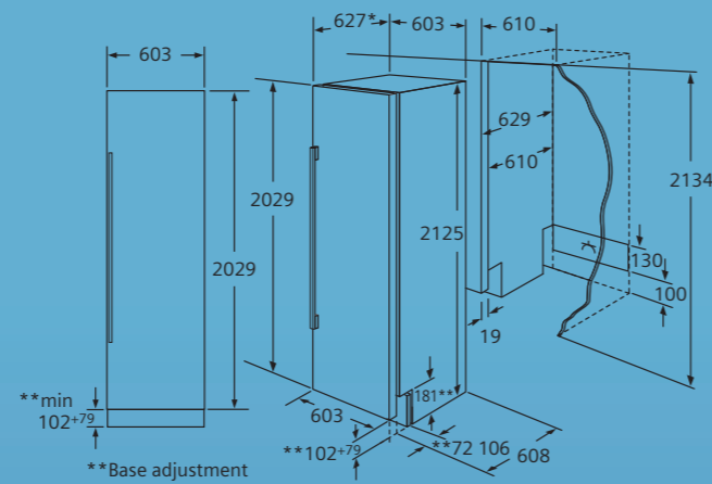
Measurements in mm
