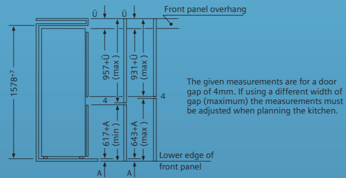
Measurements in mm
