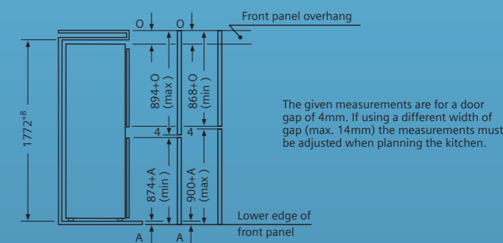
Measurements in mm
