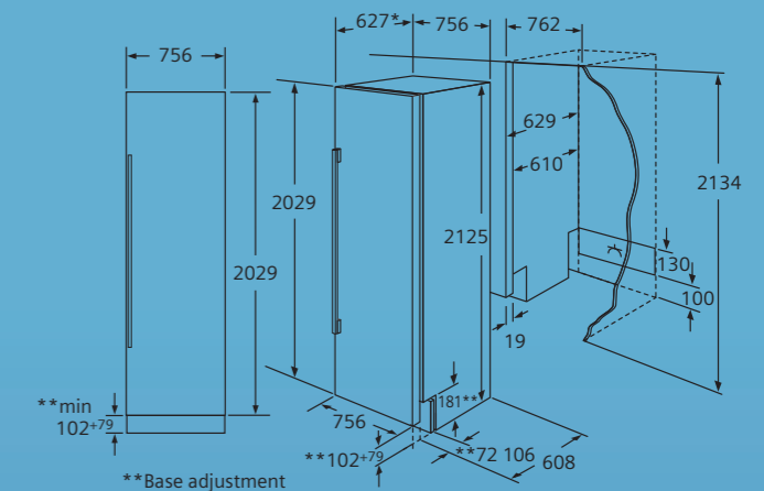
Measurements in mm
