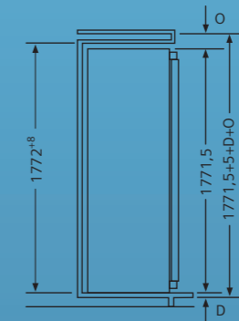
Measurements in mm
